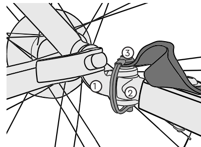
1. Hitch 2. Flex Connector 3. Retaining Pin
